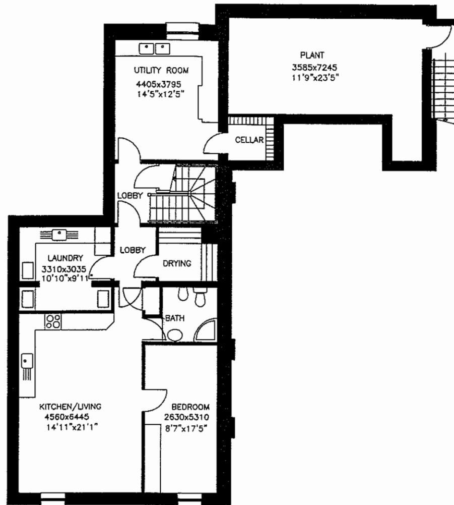
Basement Floor Plan Hanover House, Virginia Water
