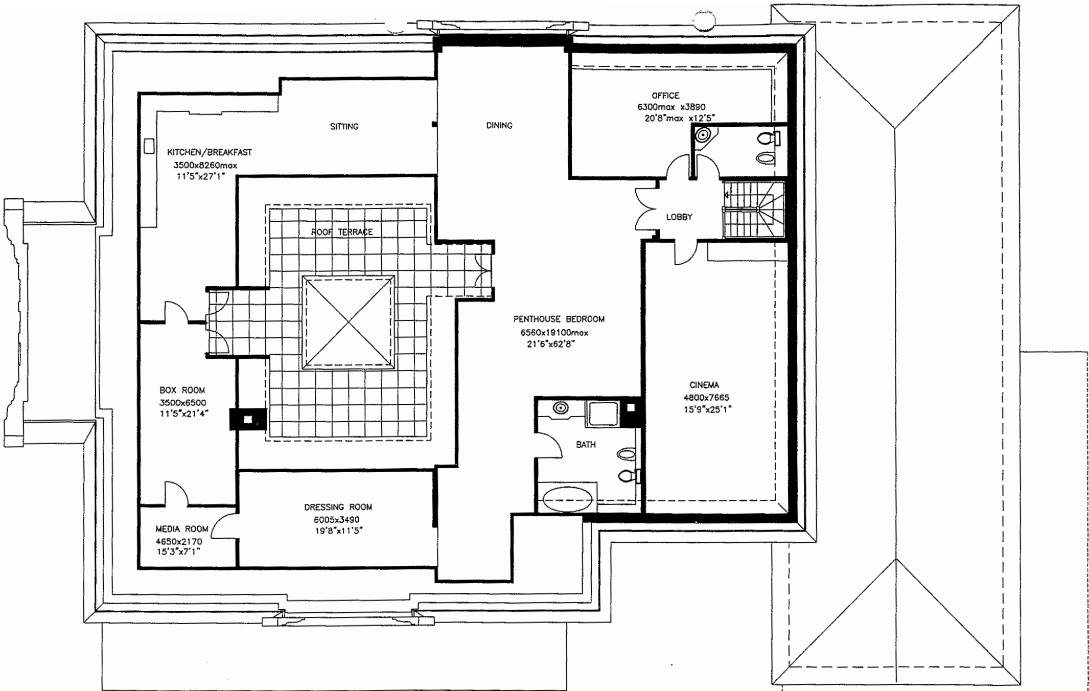
Second Floor Plan Hanover House, Virginia Water
